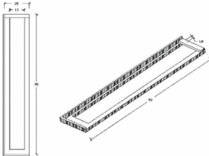
Fig. 1 Spacing mold
