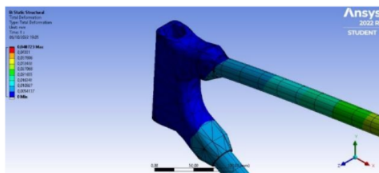
Gambar 5 Analisis Head Tube
