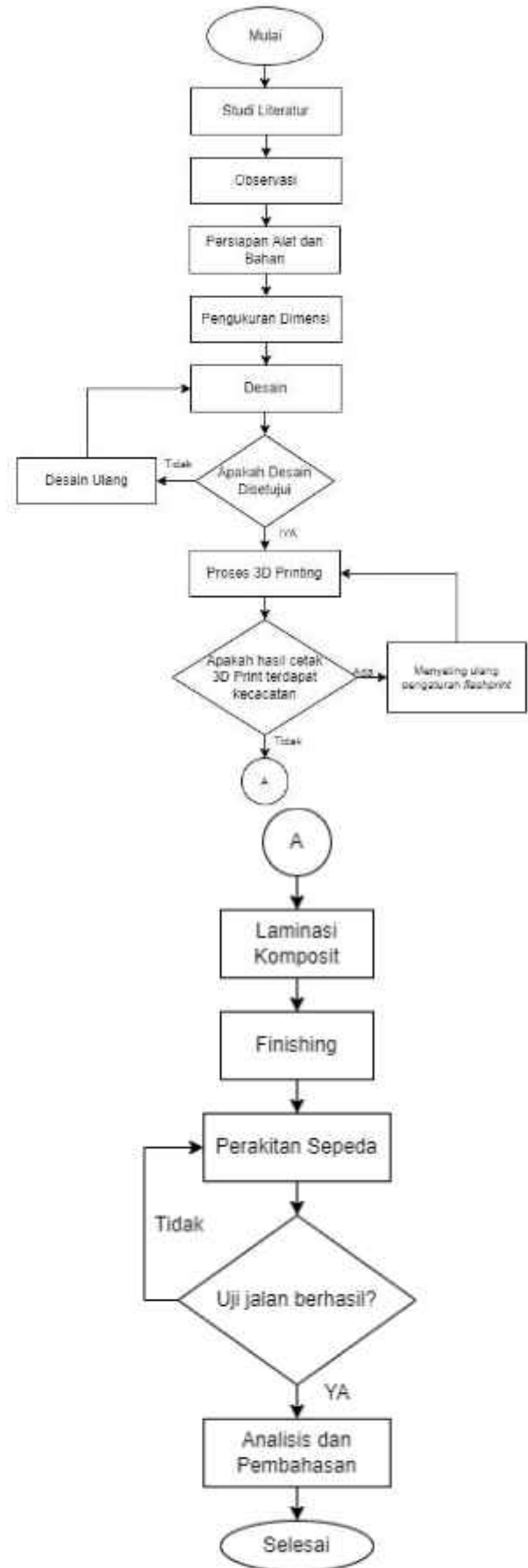
Gambar 1. Alur Penelitian.
