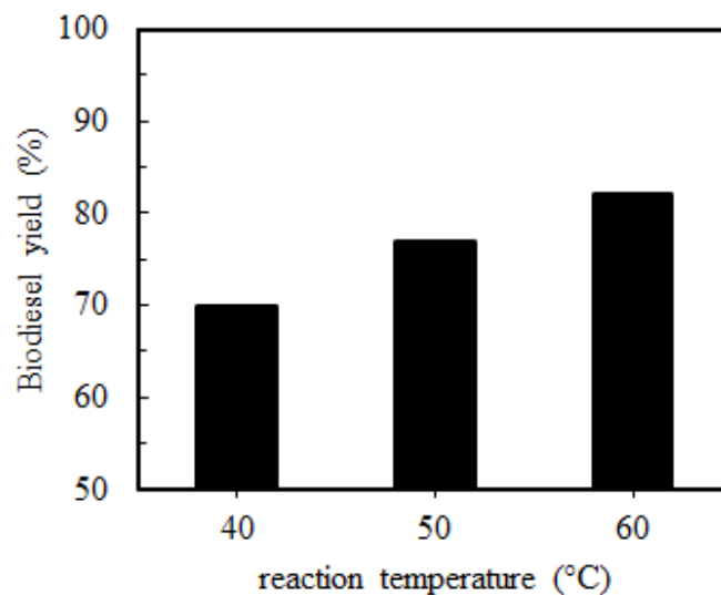
Fig. 4. Effect of Reaction Temperature on Biodiesel Yield
