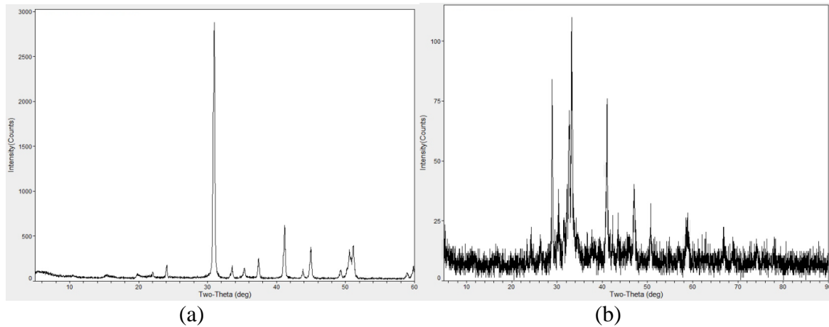
Fig. 1. The XRD Analysis Patterns of: (a) Natural Dolomite and; (b) CaO/Natural Dolomite Catalyst
