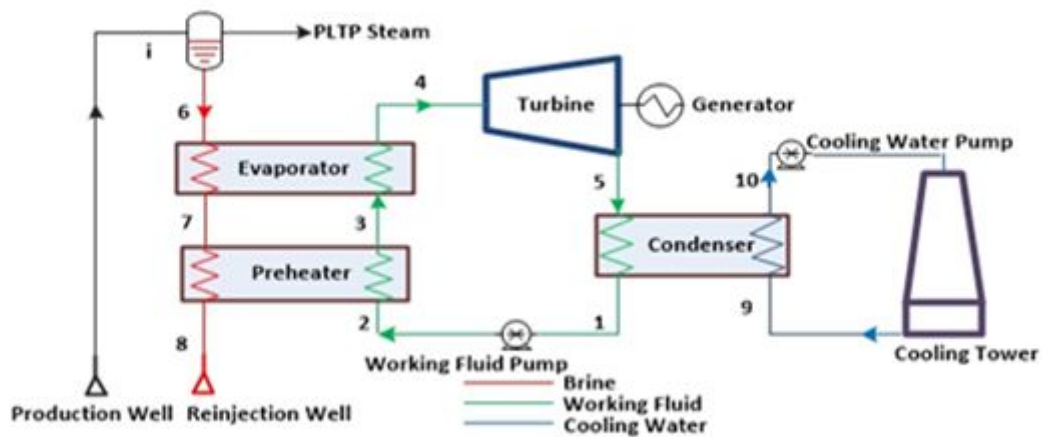
Figure 1 Schematic diagram of binary cycle system
