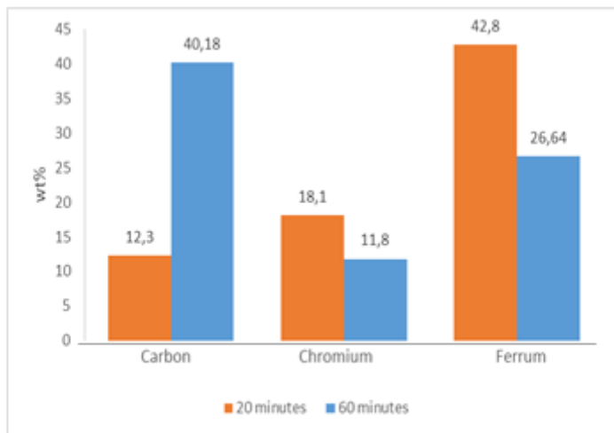
Fig. 6 EDX analysis in substrate 304 and 316 with extended of time synthesis
