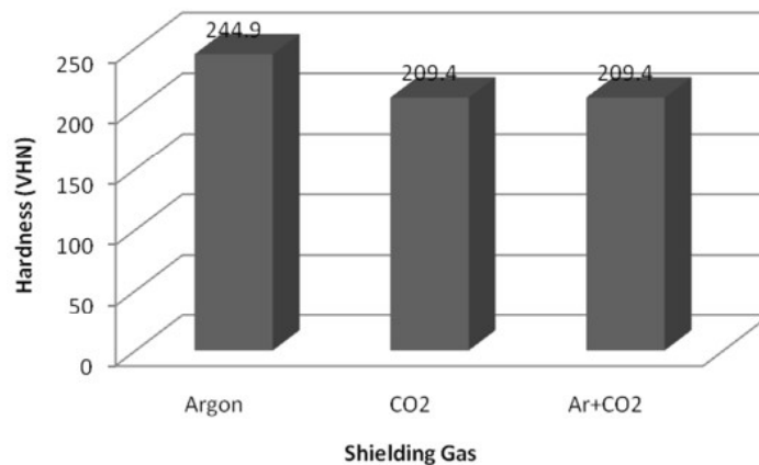
Fig. 8 Effect of Shielding Gas on Hardness
