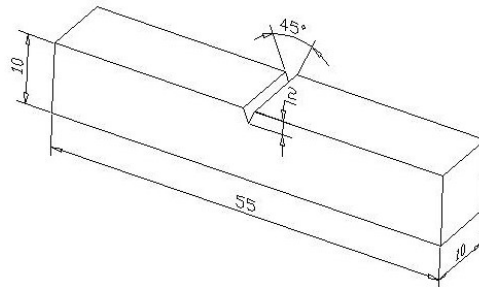
Fig. 2 Impact Test Specimen (ASTM E23-96) [5]
