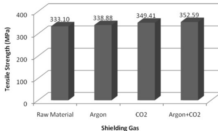
Fig. 4 Effect of Shielding Gas on Tensile Strength
