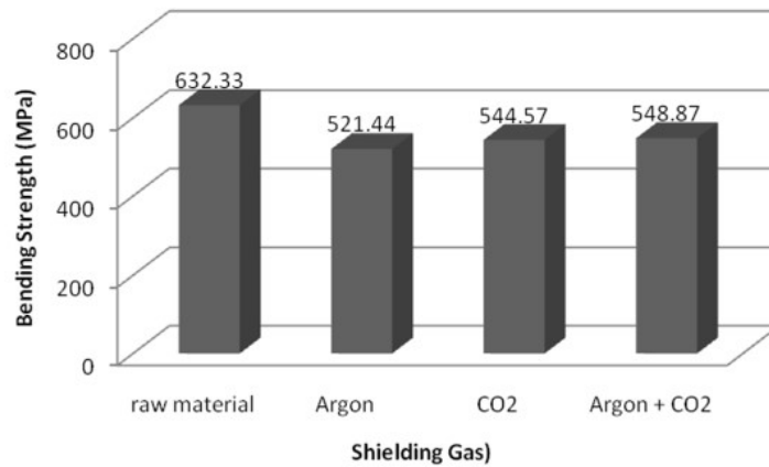
Fig. 5 Effect of Shielding Gas on Bending Strength
