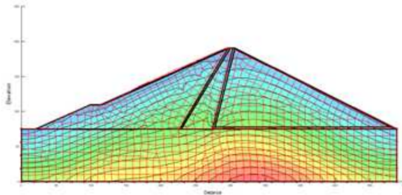
Figure 17. Deformation analysis result used SIGMA/W sub-program.
