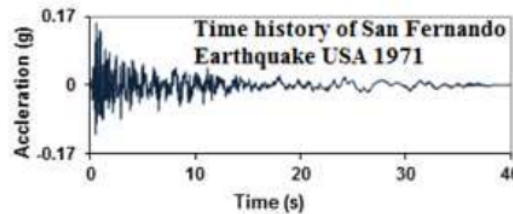
Figure 9. The time history of San Fernando earthquake USA 1971 at Santa Felita Dam station.
