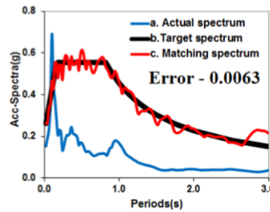
Figure 11. Spectral matching result of Figure 10 to Figure 8.
