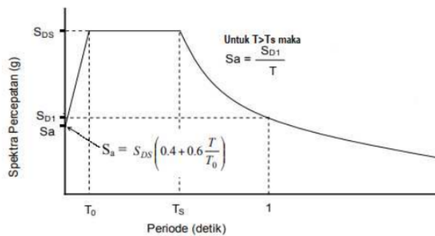
Figure 7. Design response spectrum (ASCE code 2013).
