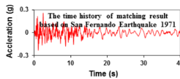
Figure 12. The artificial time history of a matching result.
