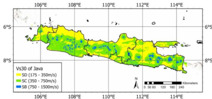
Figure 4. Soil site class (Muntafi 2021).
