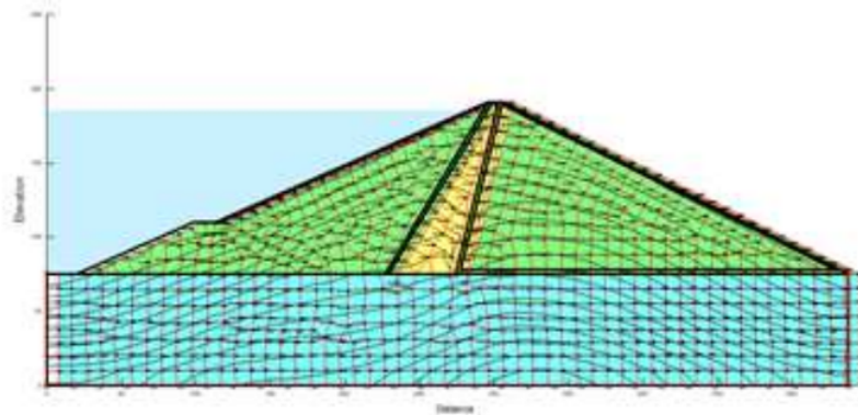
Figure 14. The dinamic response of the the Wadaslintang dam structure.
