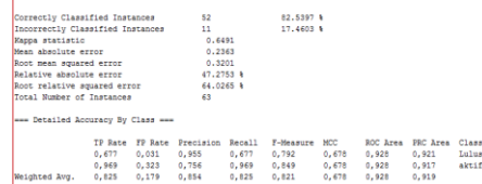
Figure 2. The classification results using the Naive Bayes method.
